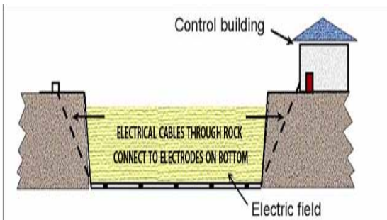
At Barriers IIA and IIB, the electric field covers 130 feet of the canal upstream to downstream. At Barrier I, the electric field covers 54 feet of the canal upstream to downstream.
